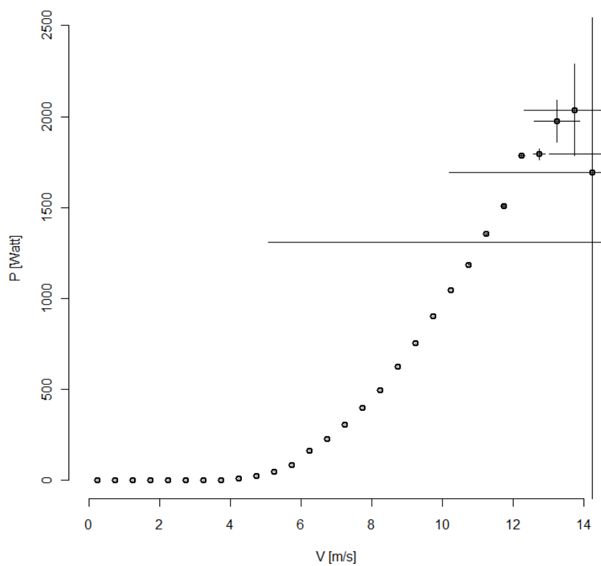
Figure 2.8: PV-curve WRE007.
